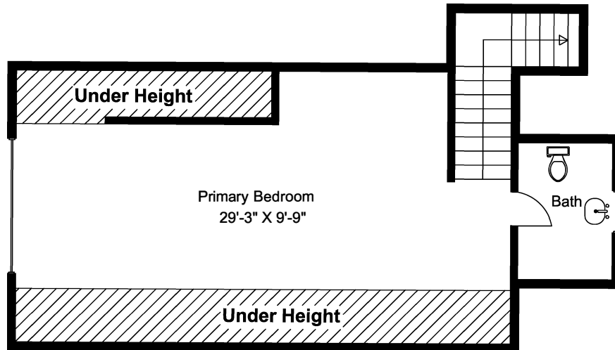
Upper Floor
